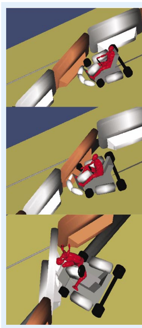
HVE simulation of three-car collision. Note that HVE shows full vehicle deformations resulting from impacts.
