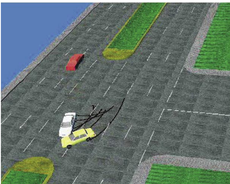
HVE simulation of two-car intersection impact.
